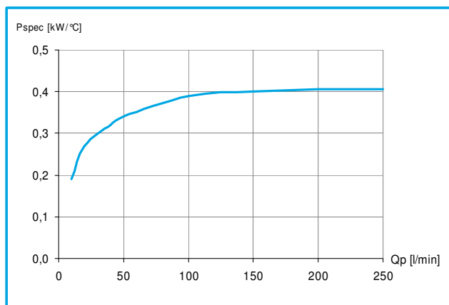
specific cooling performance
