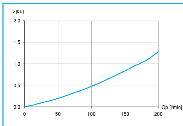
pressure drop at 30cst
